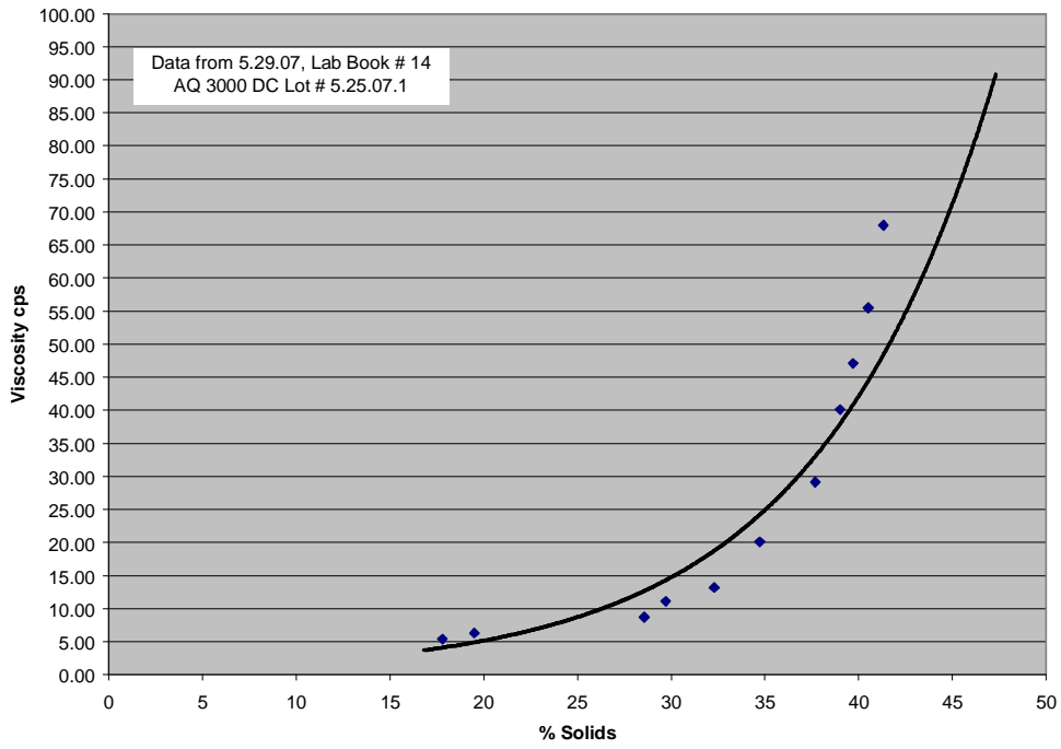
AQ 3000 DC Viscosity vs. % Solids
